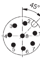
Male connector 8-pos.
