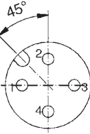
Female connector 4-pos.
