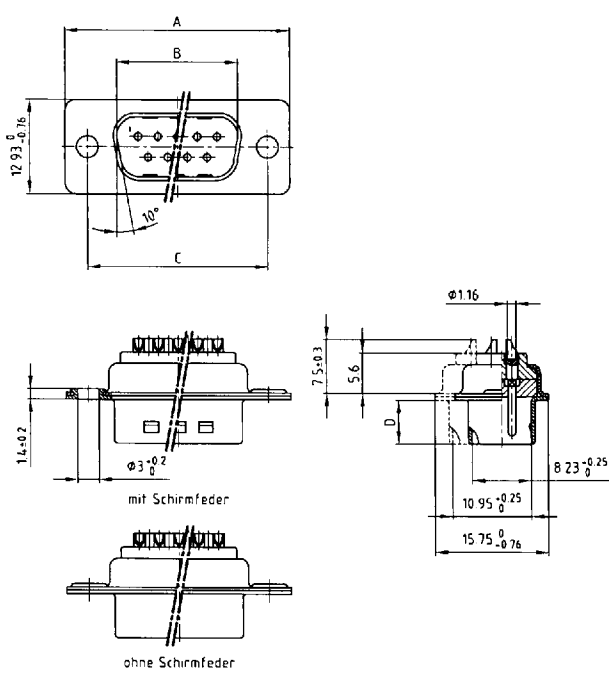
Plug connector
