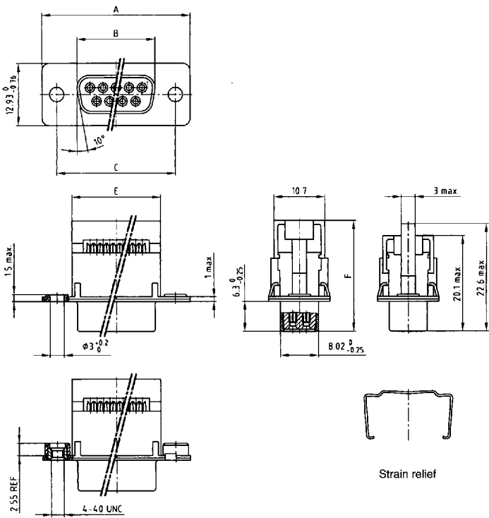
Socket connector
