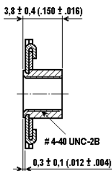
Captive Nut (E)
