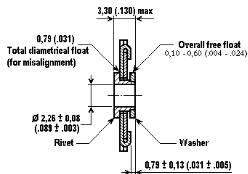
Dual Float Mount (Y)
