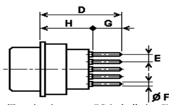
Termination type OL3 shell size F
