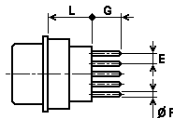
Termination type M2
