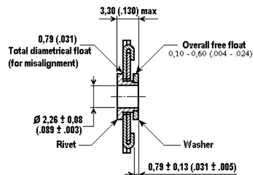
Dual Float Mount (Y)
