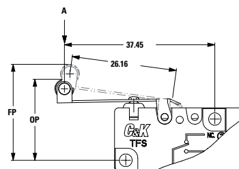
A20 Lever Roller, Low Force
