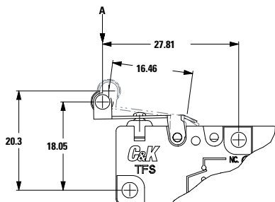
A25 Lever Roller, Low Force, Short Lever
