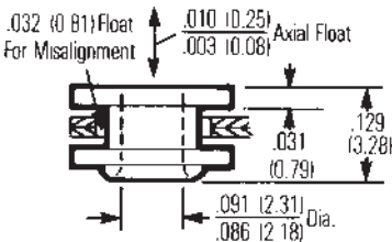
Rear panel mounting
