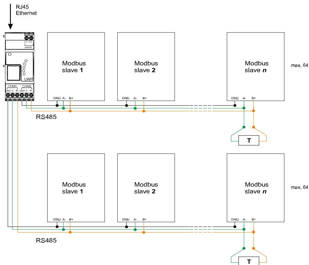
Fig. 3 Modbus RTU connection. COM 1 master, COM 2 master
