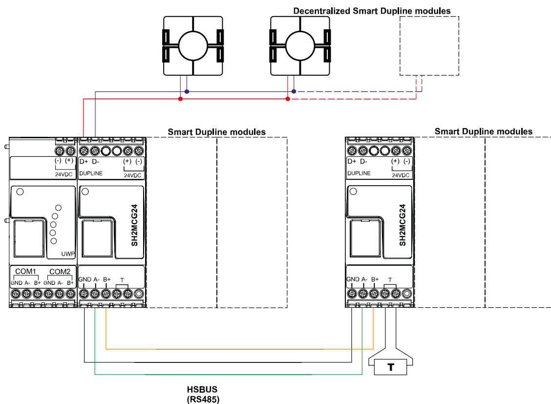
Fig. 5 Example of Smart Dupline modules connection using master channel generators
