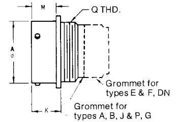
Crimp KPSE01/MS3121
