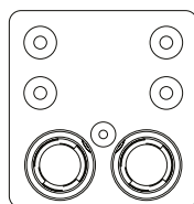
7W2 1 #16 4 #12 2 #5 Coax
