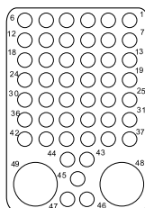
49T2 47 #20 2 #8 Triax
