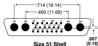
Size 51 Shell 20 Micro contacts 4 Coax or 4 Power (Not MS) 25P4 25C4
