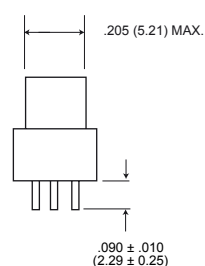
Plug
