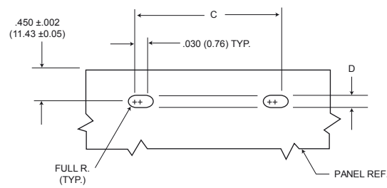
Figure 3 Edgeboard Mounting
