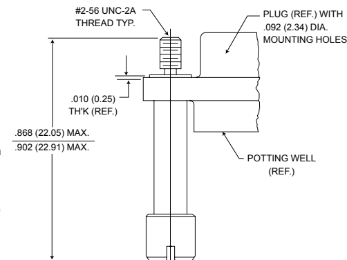
Figure 2. Jackscrew - High Profile Slotted Head Size 9-69 Size 100*
