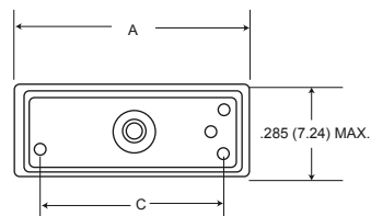
Face View
