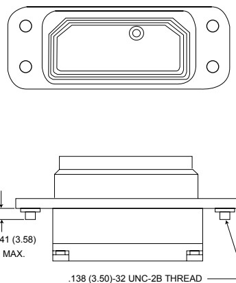
Mounting Style F Standard Hole Mounting
