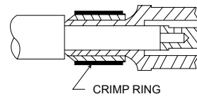
95 Ohm Contact (RG-195U) (assembly steps 1, 3, 6, 7 & 8)
