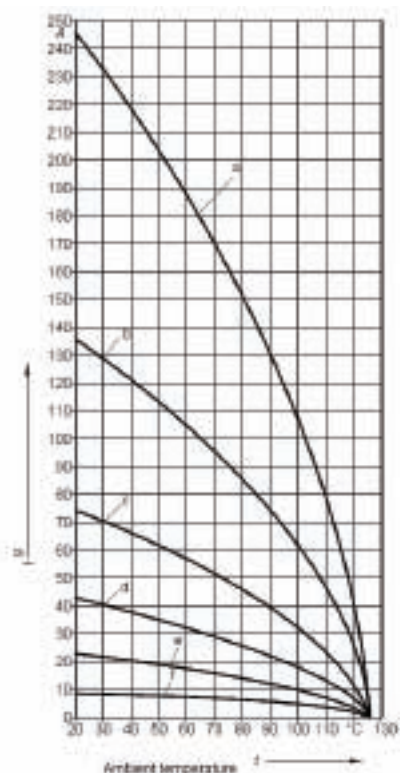
Recommended Current According to the Temperature
