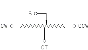
P271 (with Voltage Center Tap)
