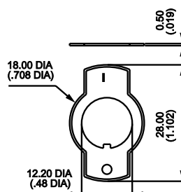
SWITCH PLATE I-O U1050 .480 I.D.
