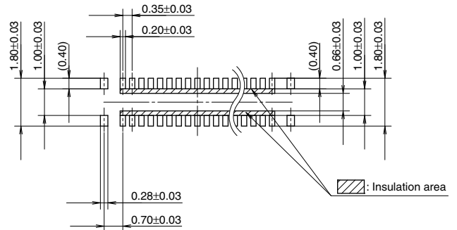
Recommended metal mask pattern
