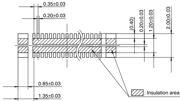
Recommended PC board pattern (TOP VIEW)
