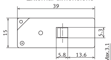
External dimensions
