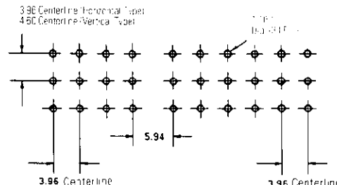
For 30 Position
