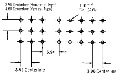
For 24 Position
