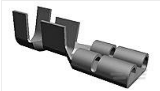
TE Part #63608-2 187 FASTON REC 20-16 AWG TPBR
