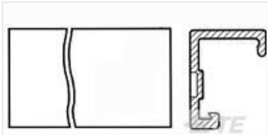
TE Part #640551-9 09P MTA156 COVER
