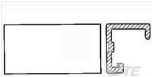
TE Part #640550-6 06P MTA100 COVER
