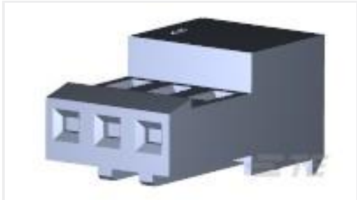
TE Part #3-641190-3 03P MTA100 CONN ASSY RED LF
