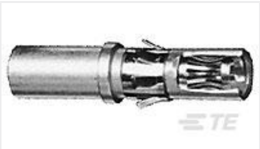
TE Part #193643-1 SKT ASSY. ,POWER, #10-12 AWG
