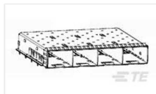
TE Part #2227730-1 zSFP+ 1x4 Cage Assembly, Press-Fit
