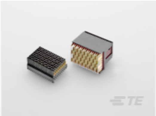
TE Part #2302789-1 VERTREACASSY,CENTER,MULTIGIG RT3
