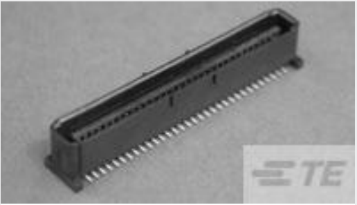
TE Part # 5146897-2 1FHP,84,30A/S,S,C,S08
