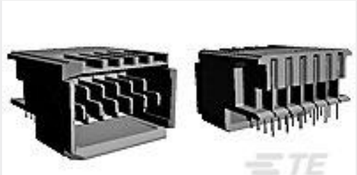
TE Part #120957-1 UPM EXPANDED PIN ASSEMBLY
