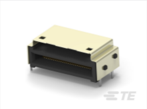
TE Part #1-2332208-3 RECEPT ASSY, RA, 56 POS, SLIVER 2.0
