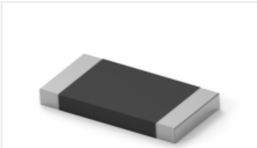
TE Part #6-2176421-3 TLRP 2512 2.0W R060 1% 50PPM 4K RL
