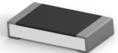
TE Part #1-2176388-3 RQ 1206 13R3 0.1% 10PPM 5K RL
