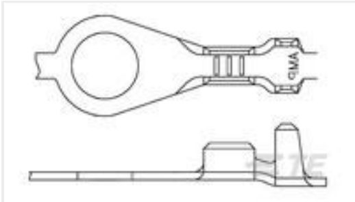
TE Part #880665-2 RING TONGUE
