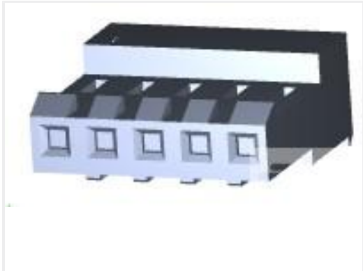
TE Part #3-640427-5 05P MTA156 CONN ASSY 20AWG YEL
