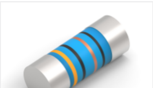
TE Part #6-2176315-6 MELF SMA_A 22K 1% 50PPM 0204 0.4 W
