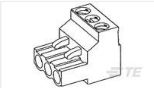
TE Part #1-796640-4 14 POS 5.0 MM R/A PLUG,TRM BLK
