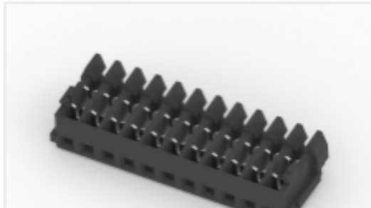
TE Part #3-353293-1 1.5MM CT MT REC ASSY 11P BLACK
