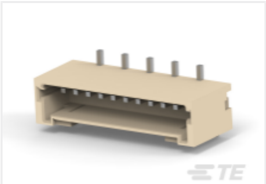
TE Part # 1-292371-1 SINGLE ROW POST HEADER ASS'Y SMT TYPE W/
