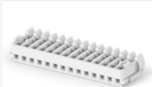
TE Part # 1-353908-4 CT REC HSG 14P CRIMP TYPE WHIT
