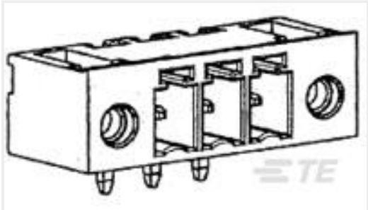
TE Part #284541-2 2 POS TERMI-BLOK 900 SF 3,81 m
