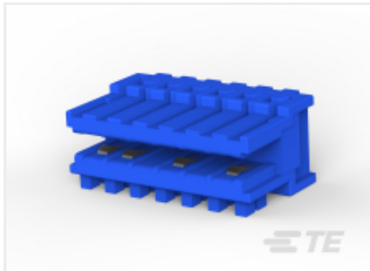
TE Part #1-284931-6 DUOPLUG 2.5 FEMALE CONN., STD, 6 POS. (S
