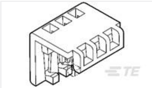
TE Part #2-643075-4 24P MTA100 MOLDED COVER
