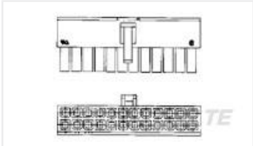
TE Part #1-1586019-6 16P RCPT VAL-U-LOK V0
