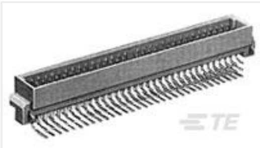
TE Part #5650947-5 ASSY, PIN, EUROCARD, TYPE C, LEAD-
