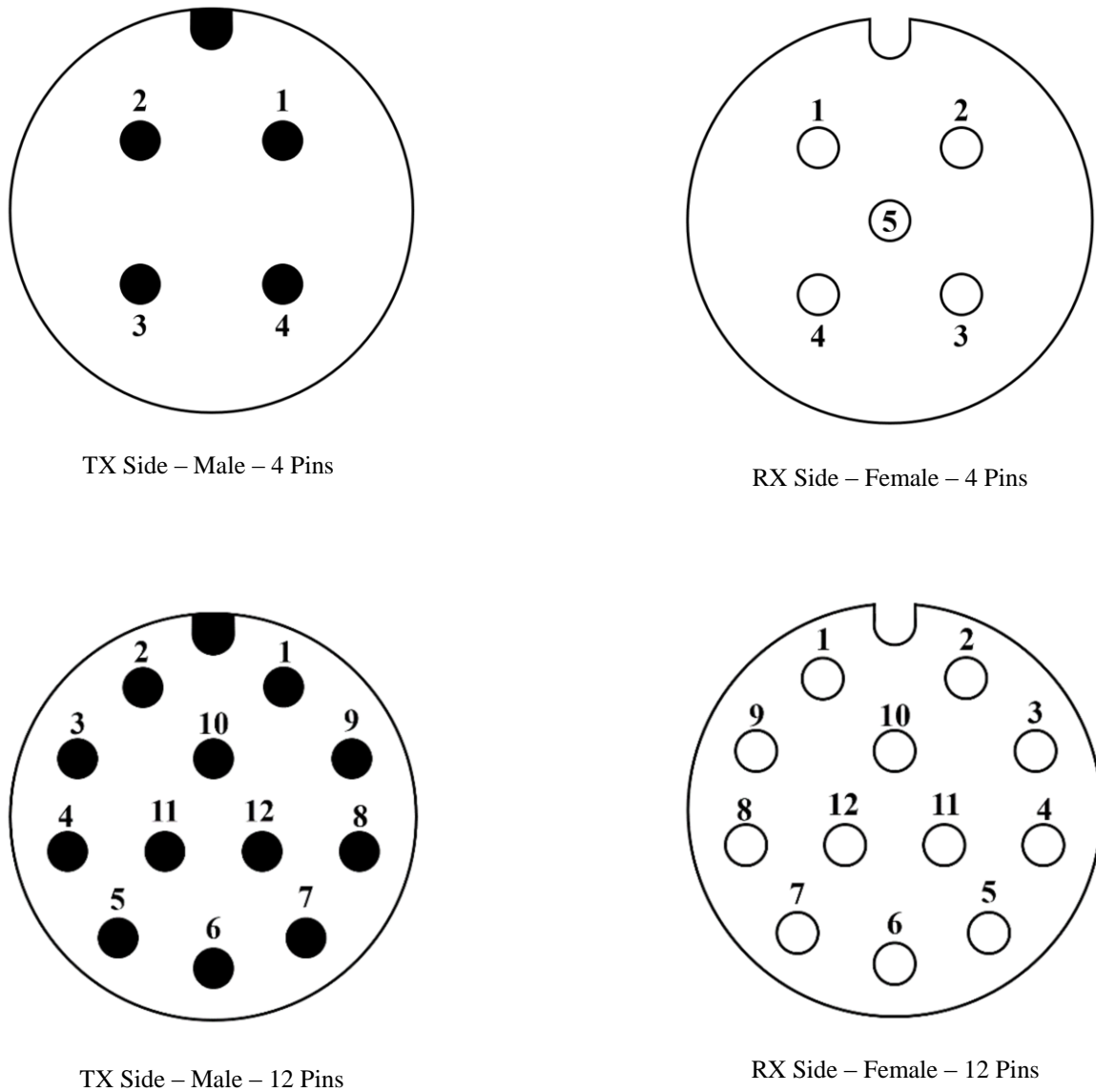
Figure 5.1 – TX and RX mating connector interfaces
