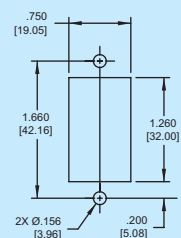
Panel Mounting Detail Mounting Detail Tolerance: ±.005 [.13] unless noted
