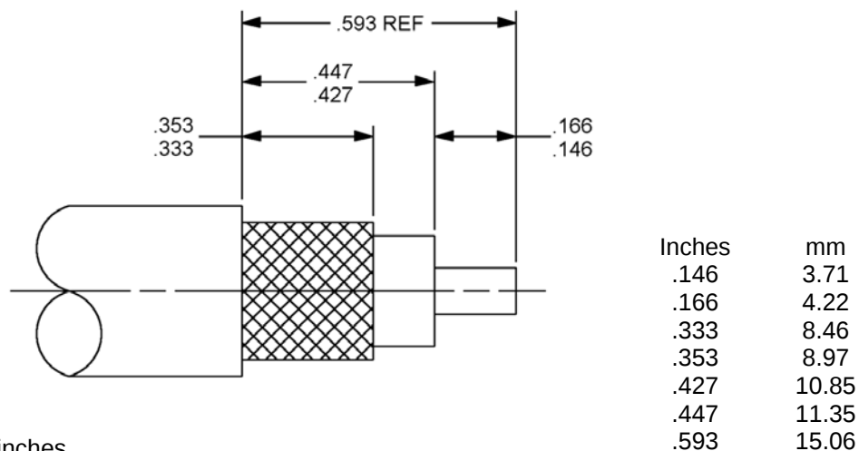
FIGURE 4. Cable stripping dimensions for field replaceable connectors.
