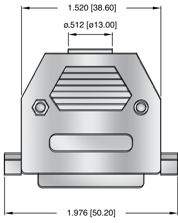
DB25-HD-PN-(SS or TS)
