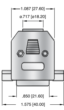
DA15-HD-PN-(SS or TS)
