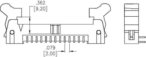
RIGHT ANGLE, THROUGH HOLE
