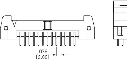
VERTICAL, THROUGH HOLE
