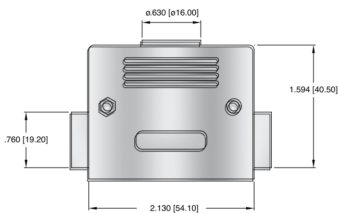
DD50-HD-PN-(SS or TS)
