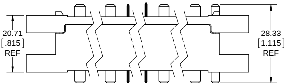
PIN AND SOCKET MATED ASSEMBLY
